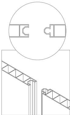
HOARDFAST HYGIENIC MODULAR PVC WALL SYSTEM
